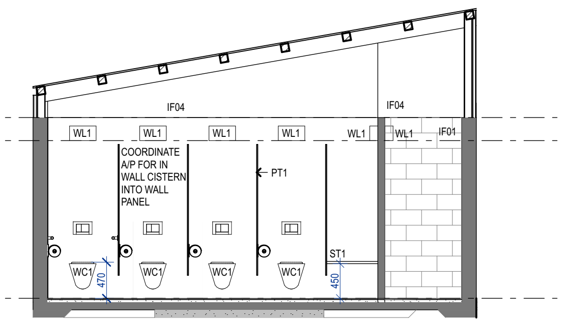
04 FEMALE AMENITIES 1:50
