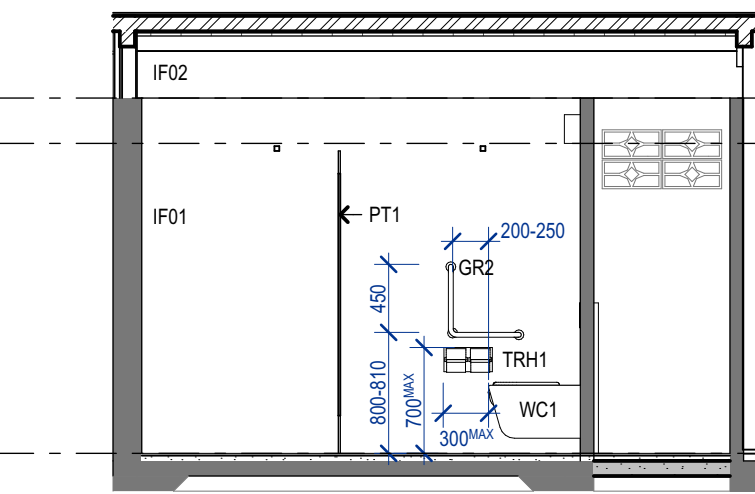
03 FEMALE AMENITIES 1:50
