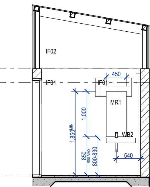
02 DDA AMENITIES 1:50
