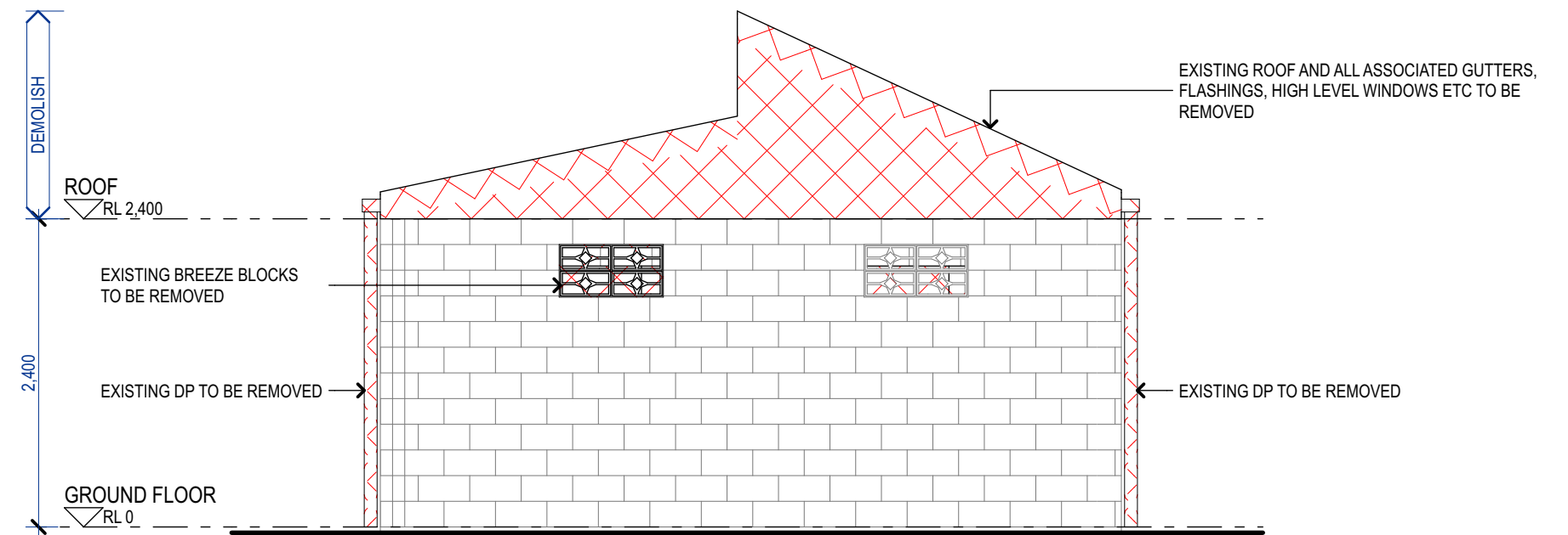
4 DEMOLITION - WEST ELEVATION 1:50
