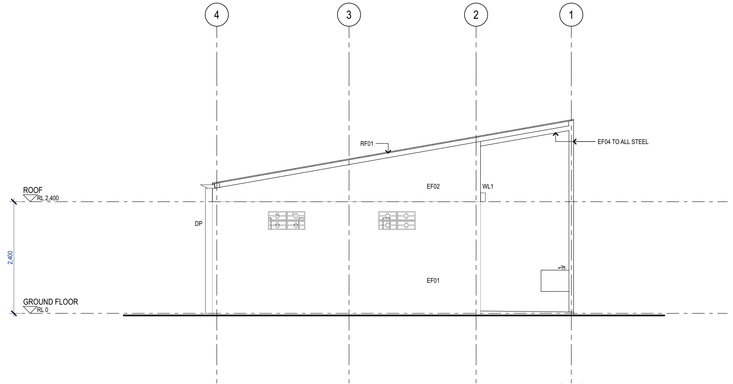
2 EAST ELEVATION - 1:50
