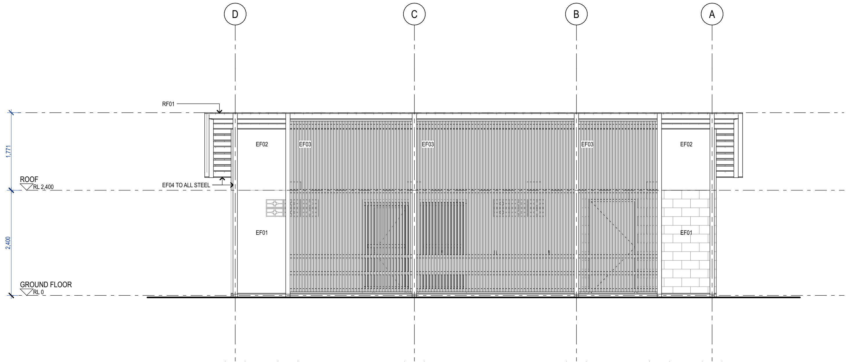
1 NORTH ELEVATION - 1:50
