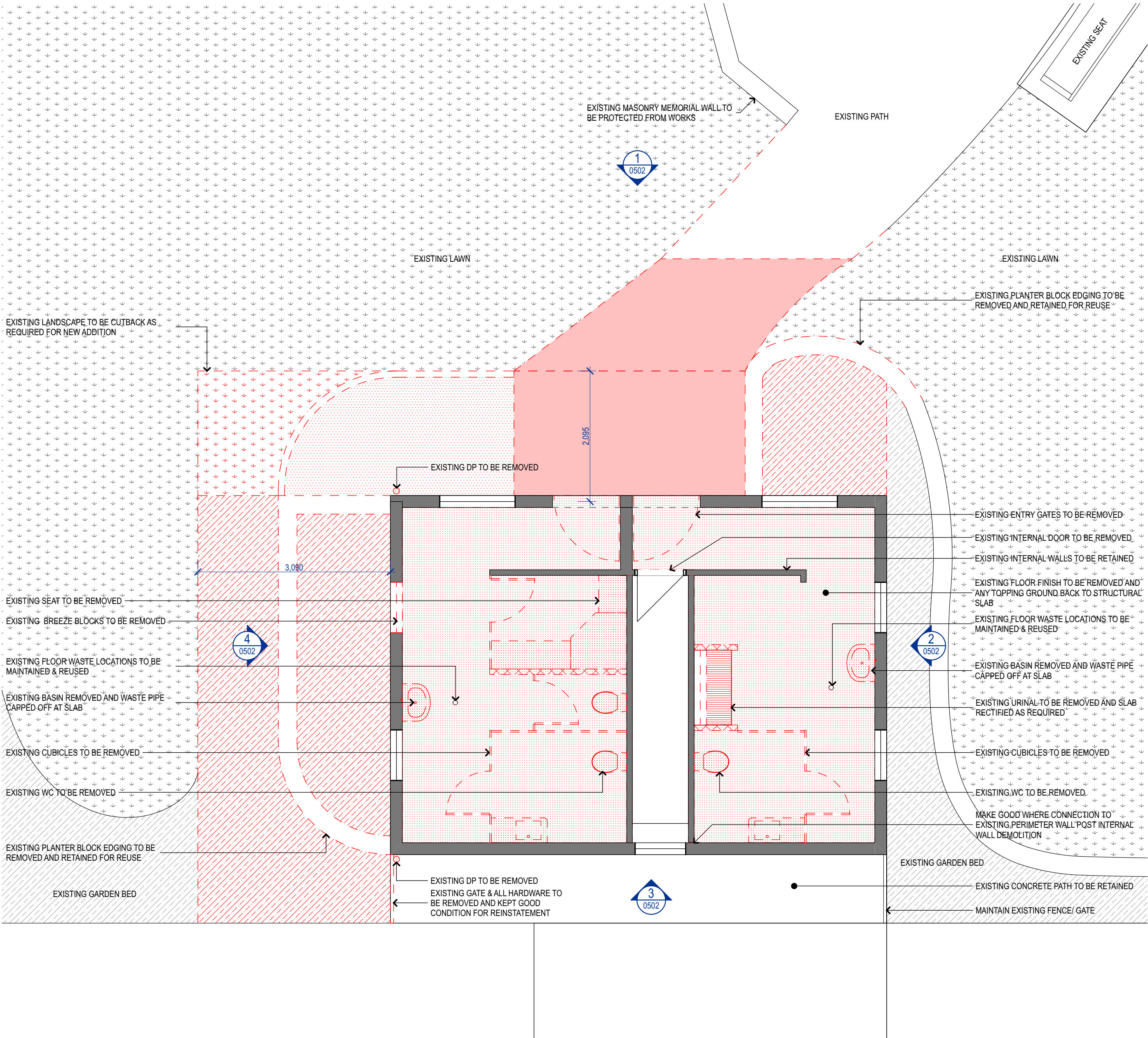
1 - 1:50 DEMOLITION PLAN - GROUND FLOOR
