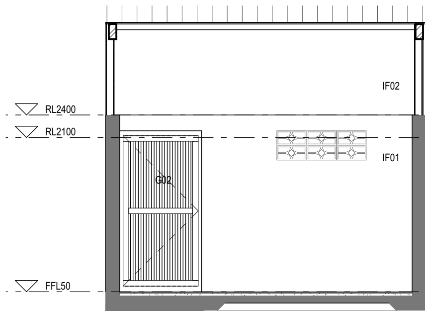
01 FEMALE AMENITIES 1:50
