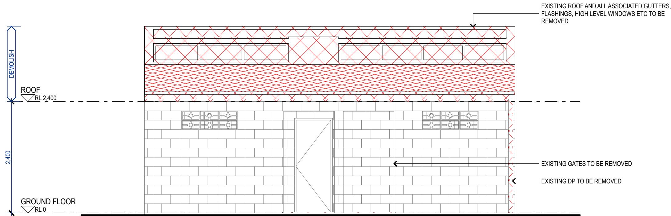
1 DEMOLITION - NORTH ELEVATION 1:50
