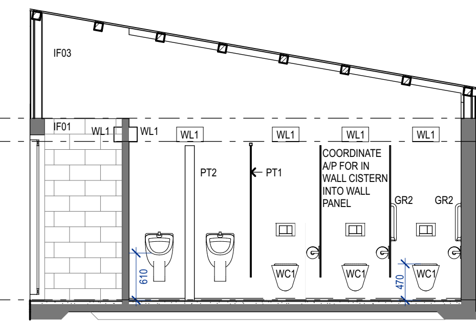
02 MALE AMENITIES 1:50
