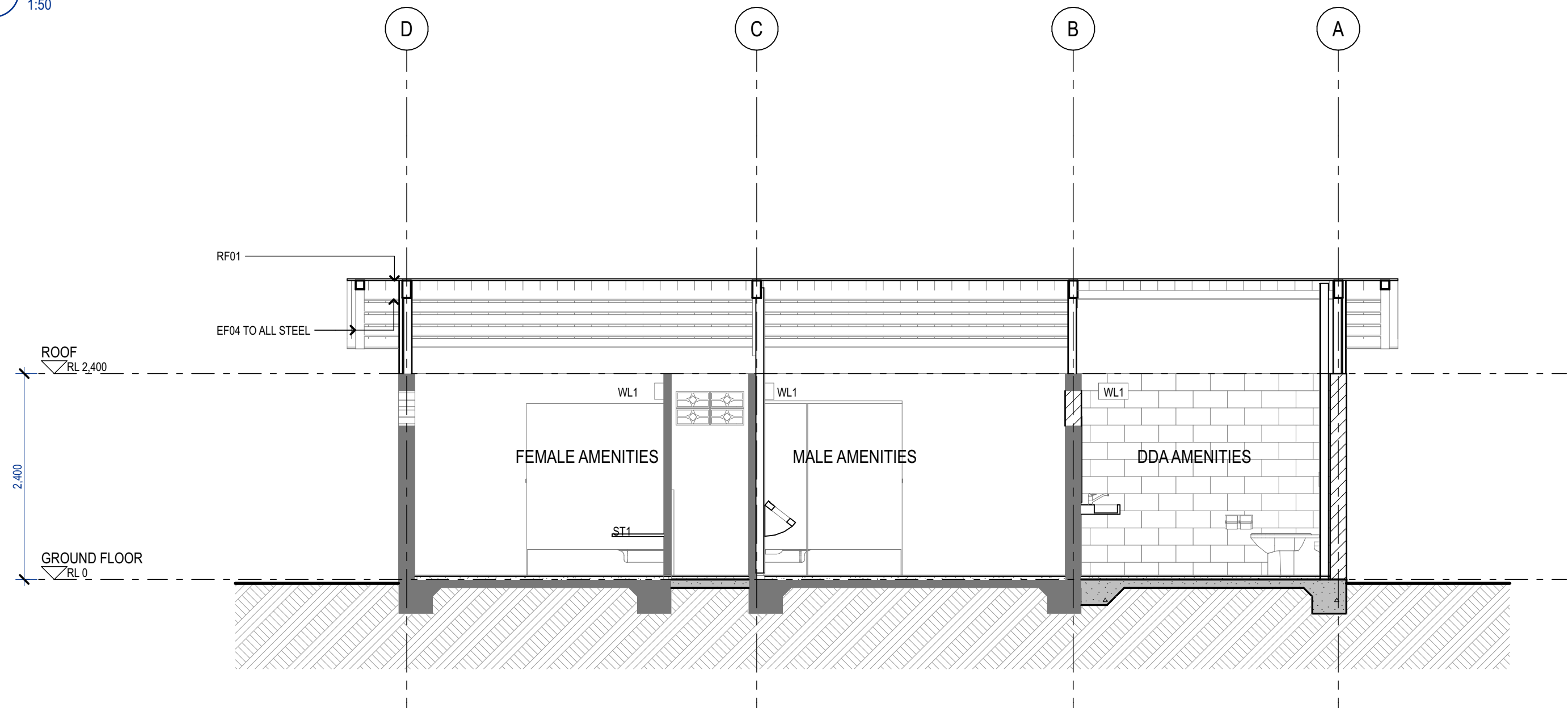
2 SECTION B - 1:50
