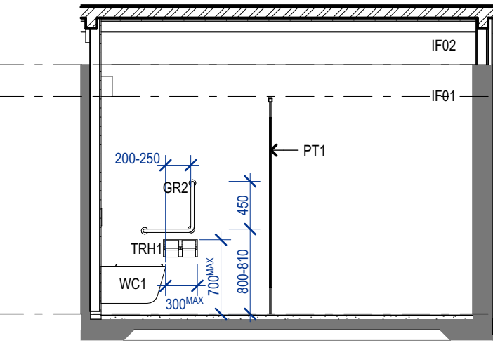
03 MALE AMENITIES 1:50
