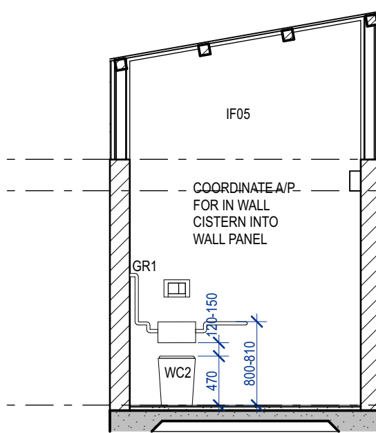
04 DDA AMENITIES 1:50
