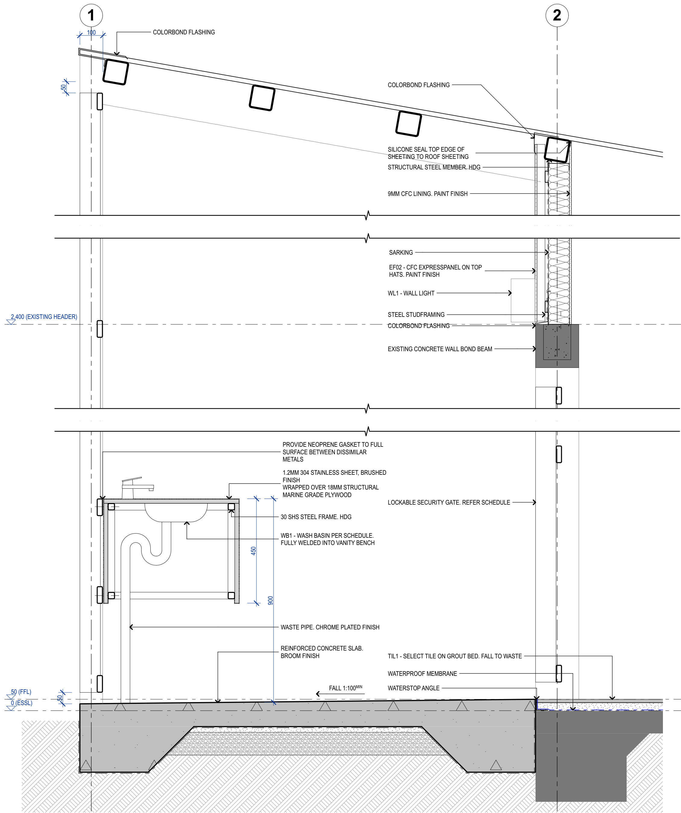
1 SECTION DETAIL 1:10
