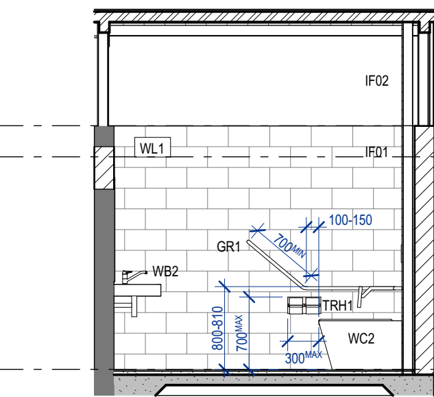
03 DDA AMENITIES 1:50
