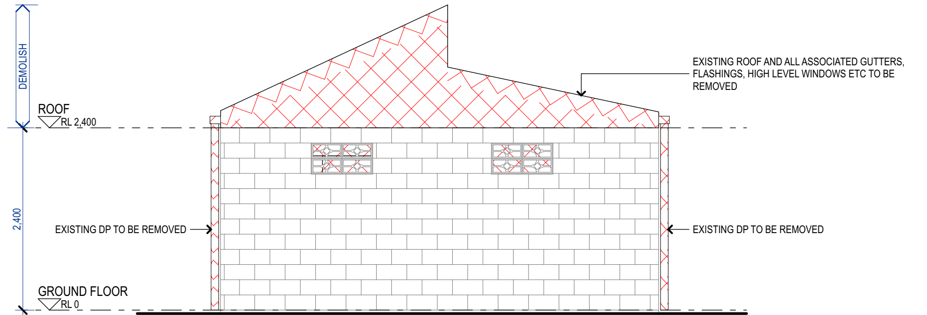
2 DEMOLITION - EAST ELEVATION 1:50
