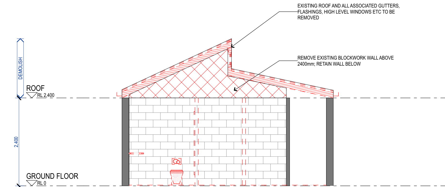
5 DEMOLITION - INTERNAL ELEVATION (1) 1:50
