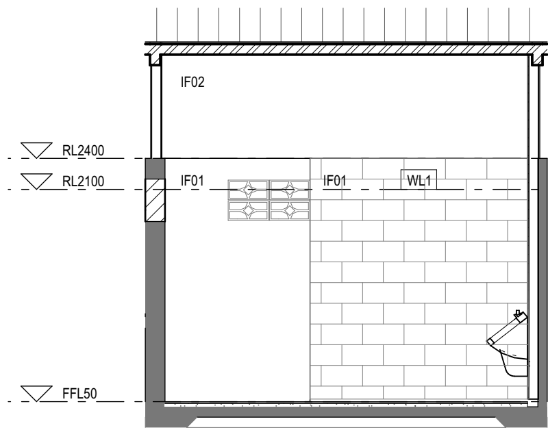
01 MALE AMENITIES 1:50
