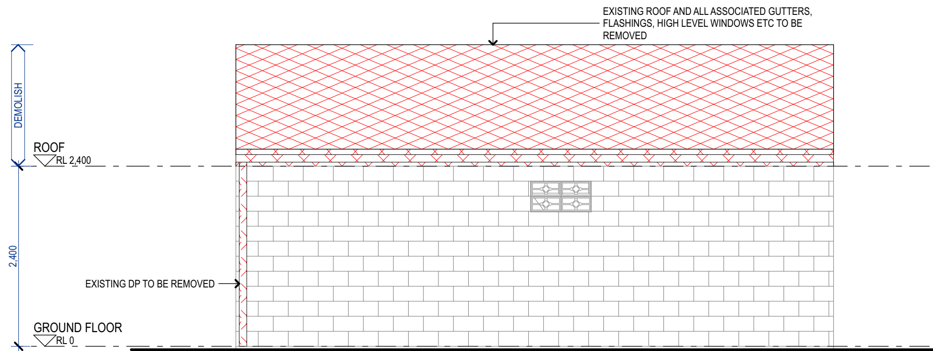
3 DEMOLITION - SOUTH ELEVATION 1:50
